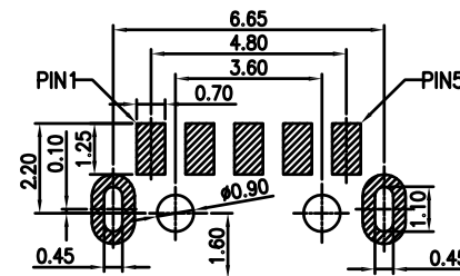
Recommended P.C.B. Layout General tolerance: ±0.05mm
