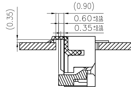
SMT AFTER SCALE 2:1
