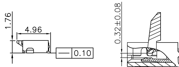
OPEN POSITION SCALE 2:1
