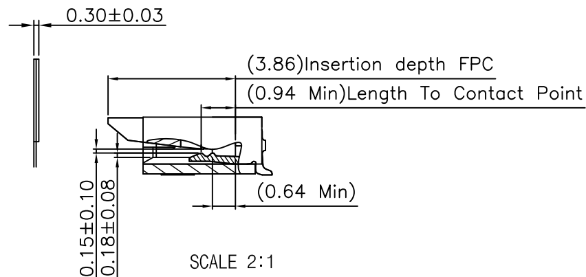
OPEN POSITION SCALE 2:1
