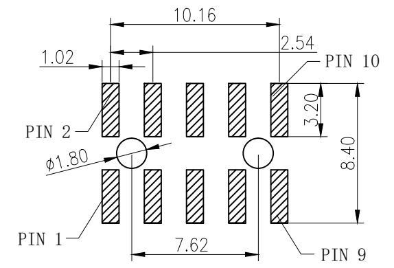
Recommended P.C.B. Layout Total tolerance:±0.05mm
