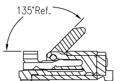
When Actuator Is Opened Scale 2:1
