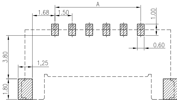
Recommended P.C.B. Layout Total tolerance:±0.05mm
