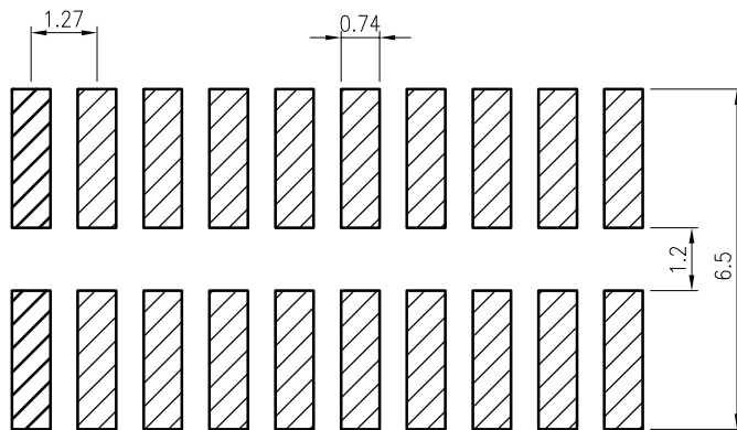
Recommended P.C.B. Layout General tolerance: ±0.05mm
